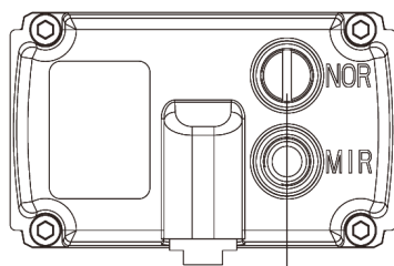
Magnet Screw
